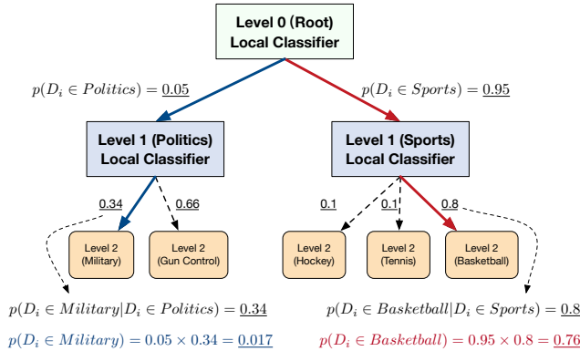
Figure 1: Ensemble of local classifiers.
