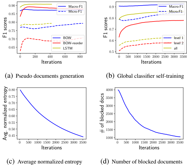
Figure 2: Component-wise evaluation on NYT dataset.
