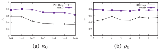
Figure 6: Comparison Results with Various Geo Parameter Settings
